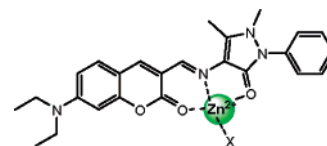
Figure 4. Proposed interaction mode between L and Zn 2+ .
