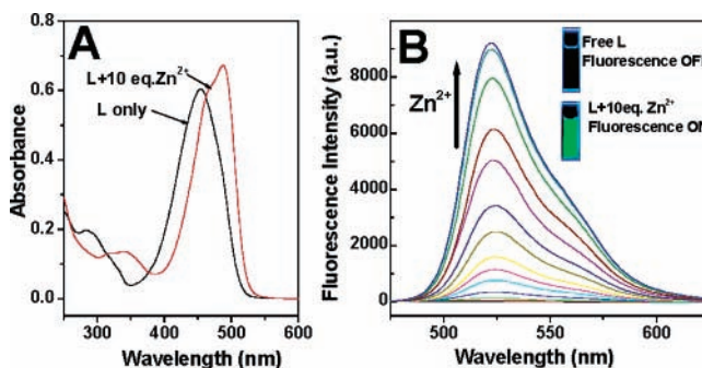
Figure 3. (A) UV–vis spectra of L (10 μM) and L (10 μM) upon addition of 10 equiv of Zn(ClO 4 ) 2 in CH 3 CN. (B) Fluorescence spectra of L (10 μM) in CH 3 CN upon addition of increasing concentrations of Zn(ClO 4 ) 2 (0, 2.5, 5, 7.5, 10, 15, 20, 30, 40, 50, 60, 70, 80, 90, and 100 μM) with an excitation wavelength of 450 nm. Inset: Photos of L in CH 3 CN with and without addition of Zn(ClO 4 ) 2 .
