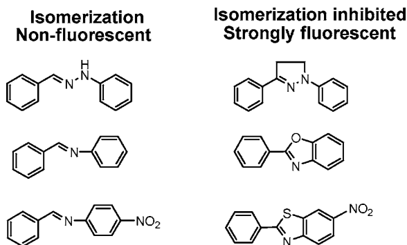
Figure 1. Molecular structures of unbridged and bridged C=N compounds.
