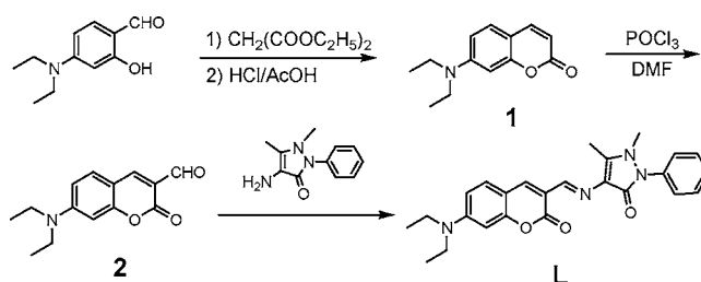
Figure 2. Synthetic method of compound L .
