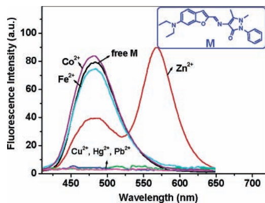
Figure 5. Fluorescence spectra of M (10 \mu\text{M} ) in \text{CH}_3\text{CN} upon addition of different metal cations including \text{Zn}^{2+} , \text{Cu}^{2+} , \text{Hg}^{2+} , \text{Pb}^{2+} , \text{Fe}^{2+} , and \text{Co}^{2+} (each concentration was 100 \mu\text{M} ) with an excitation wavelength of 400 nm. Inset: molecular structure of M .
